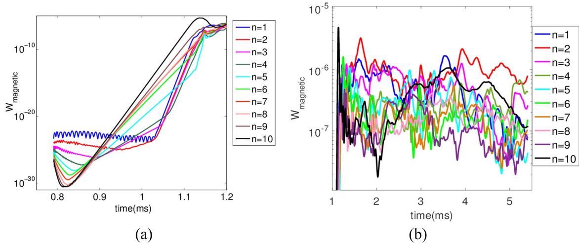
Figure 3. Time evolution of the perturbed magnetic energy in arbitrary units for toroidal modes n = 1 – 10 at the linear growth phase (a) and at the saturation phase (b) for the original (experimental) #145117 plasma equilibrium.
