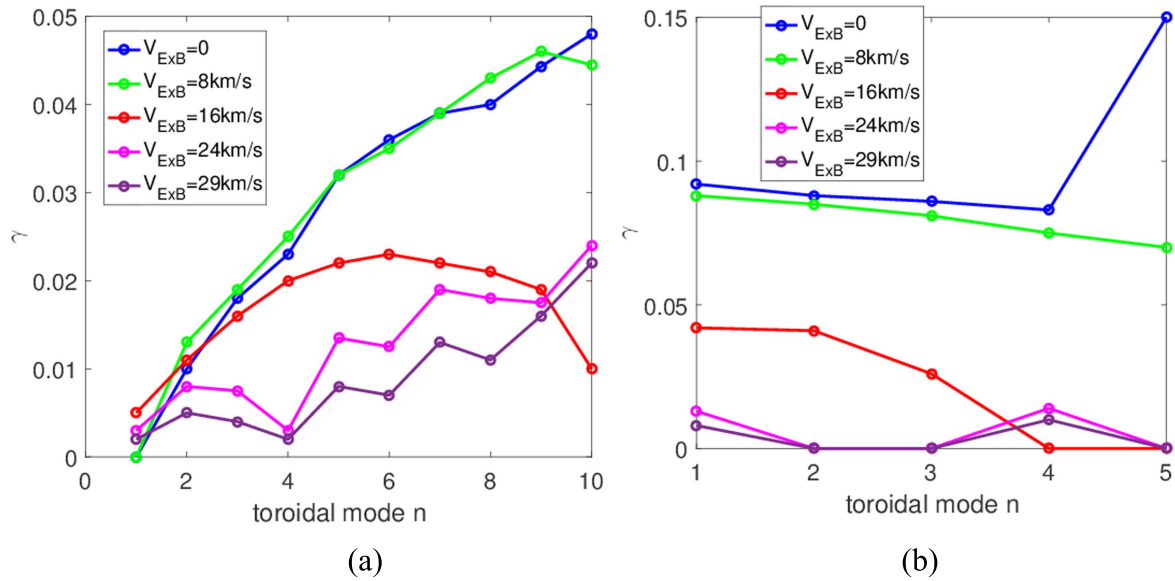
Figure 16. (a) Linear growth rate of toroidal modes n = 1-10 with different V_{ExB} rotation speed at the edge of the plasma. (b) nonlinear growth rate of toroidal modes n = 1-5 with different V_{ExB} rotation speed at the edge of the plasma. The growth rate \gamma is normalised by \sqrt{\mu_0 \rho_0} .
