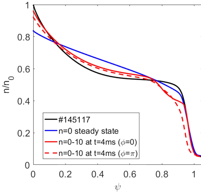
Figure 10. Density profiles for n = [0-10] at t = 4 ms (see figure 9).
