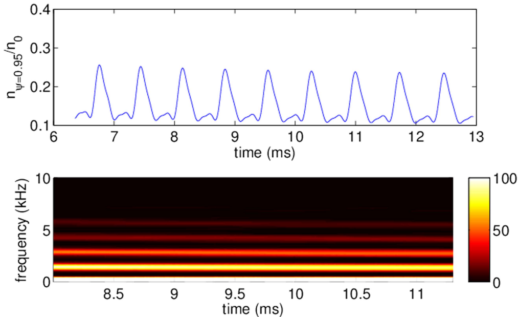
Figure 1. Density fluctuation due to the kink-peeling mode (EHO) at the outer mid-plane during the saturation phase 6–13 ms from the nonlinear MHD simulation.
