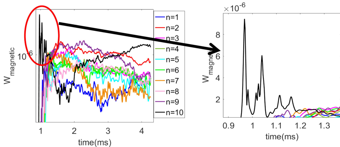
Figure 9. Time evolution of the perturbed magnetic energy of toroidal modes n = 1-10 during the saturation phase for the simulation of the modified equilibrium plasma with lower edge current and higher pedestal pressure.
