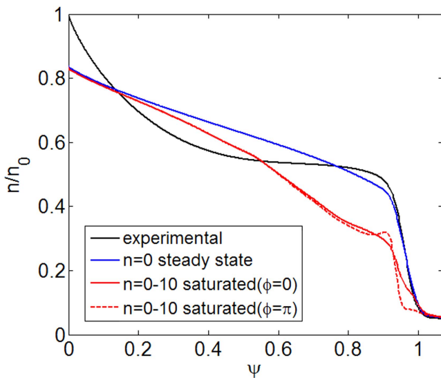
Figure 4. Density profiles for n = [0-10] during the saturation phase at t = 3.0 ms.
