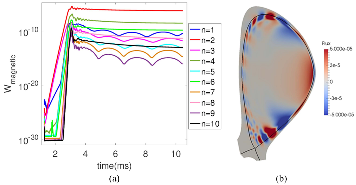
Figure 14. (a) Time evolution of the perturbed magnetic energy of toroidal modes n = 1-10 with edge E \times B speed V_{E \times B} = 24 \text{ km s}^{-1} ; (b) contour plot of flux for the perturbation of n = 1-10 modes in the poloidal plane (separatrix in black) during the saturation phase of the simulation with edge E \times B speed V_{E \times B} = 24 \text{ km s}^{-1} .
