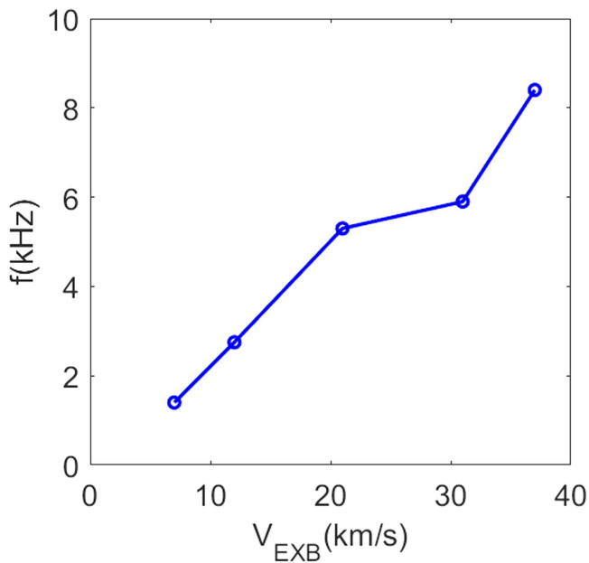
Figure 15. KPM rotation frequency in the poloidal plane in the counter clockwise direction versus edge E \times B speed.
