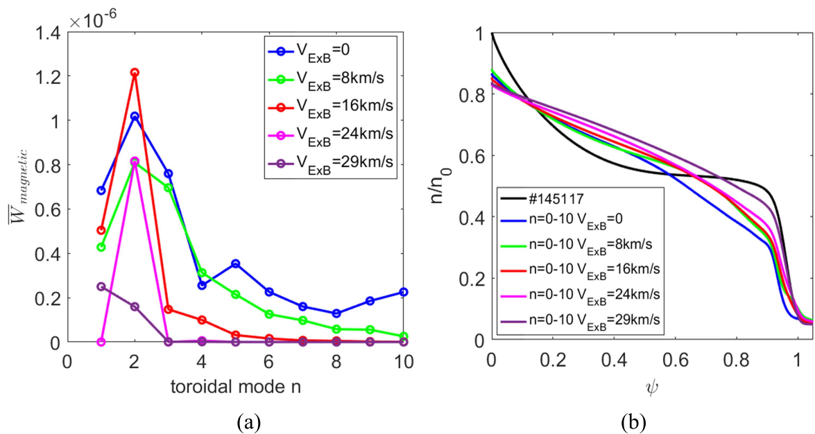
Figure 17. (a) Time-averaged magnetic energy of each mode n = 1-10 through the stationary phase for different edge V_{ExB} speeds; (b) density profiles in the saturation phase with different edge V_{ExB} speeds for simulations including modes n = 0-10 at toroidal phase \phi = 0 .
