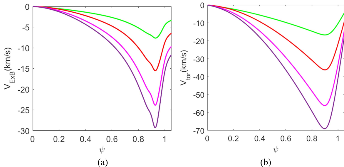
Figure 13. Profiles of V_{E \times B} rotation (a) and toroidal rotation (b) with different rotation speeds at the edge of the plasma in the equilibria modelled with JOREK.
