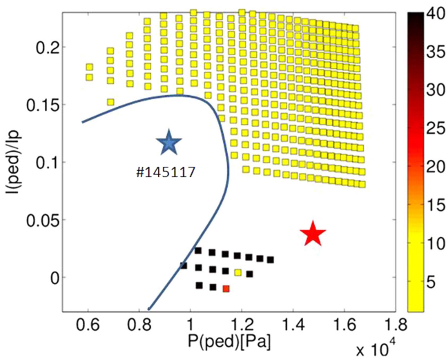
Figure 7. Linear ideal MHD stability diagram of the pedestal plasma in DIII-D QH-modes. The blue star represents the equilibrium of the DIII-D QH-mode plasma #145117, the red star is the modified equilibrium with lower edge current and higher pedestal pressure. The colour code indicates the toroidal mode number of the most unstable mode.
