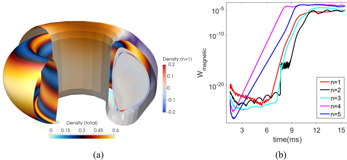
Figure 18. (a) 3D density structure at the separatrix and resistive wall potential of an n = 1 saturated KPM in an ITER Q = 10 plasma. (b) Time evolution of the perturbed magnetic energy for the n = 1 –5 modes for an ITER Q = 10 plasma.
