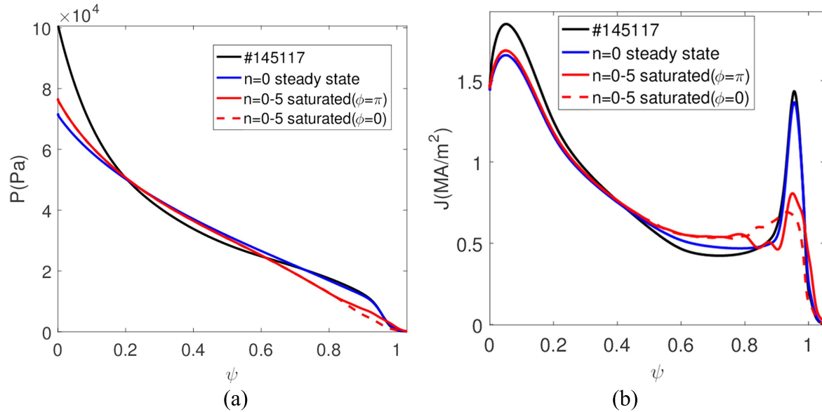
Figure 2. Profiles of pressure (a) and current density (b) before and during the KPM saturation phase.
