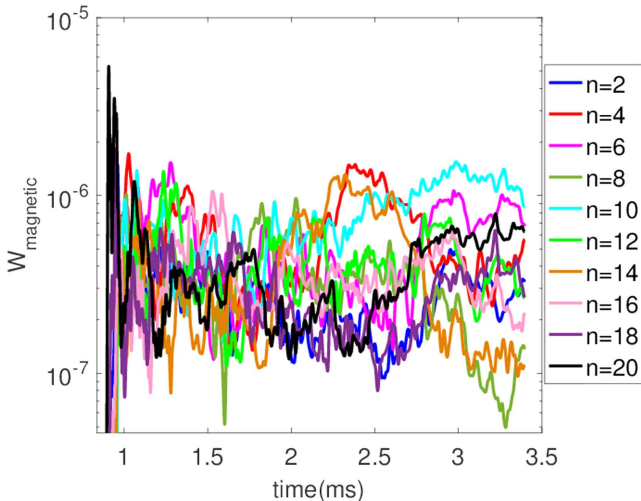
Figure 11. Time evolution of the perturbed magnetic energy of even number modes n = 2-20 in the saturation phase for the simulation of the modified equilibrium with lower edge current and higher pedestal pressure.
