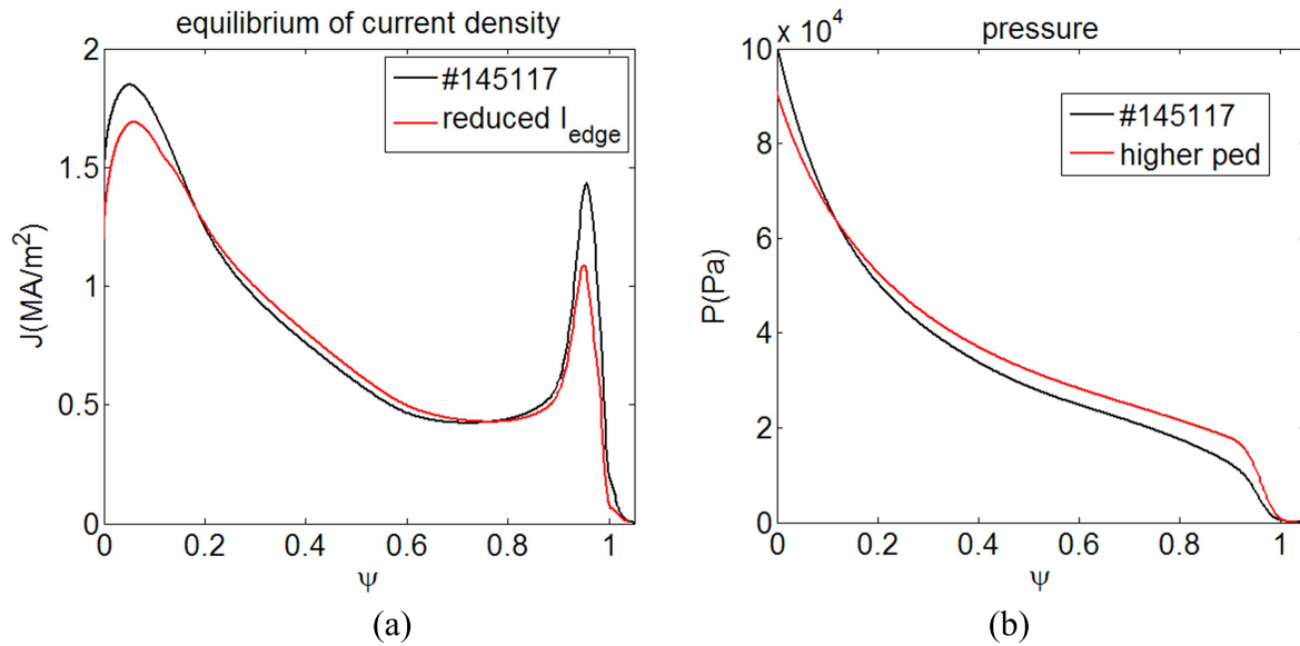
Figure 8. (a) Current profiles and (b) pressure profiles; initial equilibrium profile of the experimental plasma (black curve) and of the modified equilibrium (red curve).
