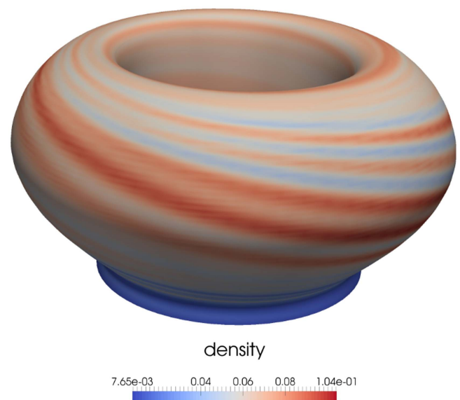
Figure 5. 3D helical structure of the density perturbation for the saturated n = 1 – 10 modes at the separatrix from the JOREK simulation at t = 3.0 ms.
